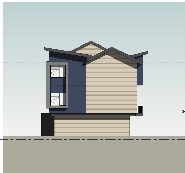
③ North 1/8" = 1'-0"
