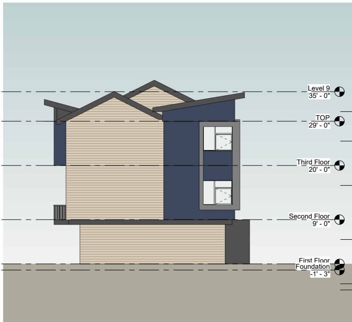
④ South 1/8" = 1'-0"
