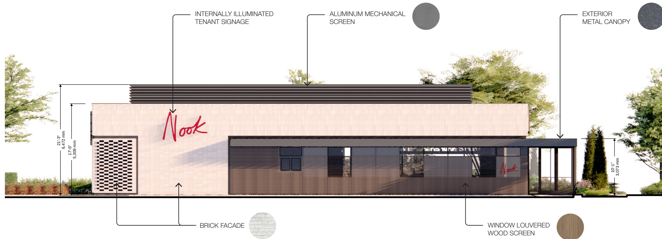
North Elevation
