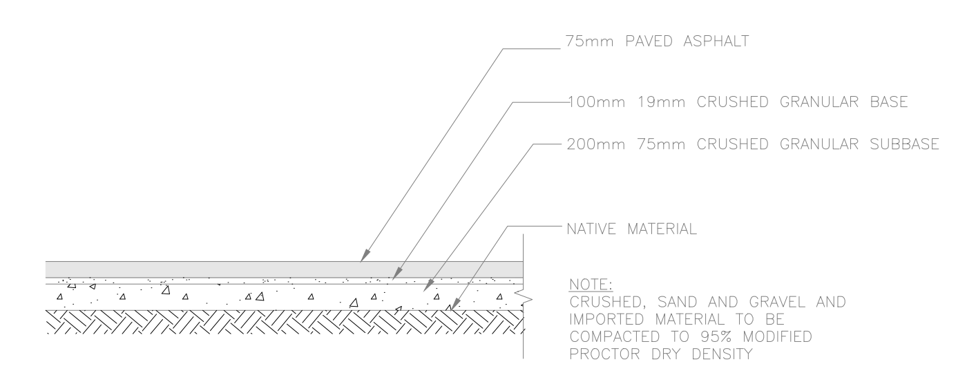
PAVEMENT DETAIL
